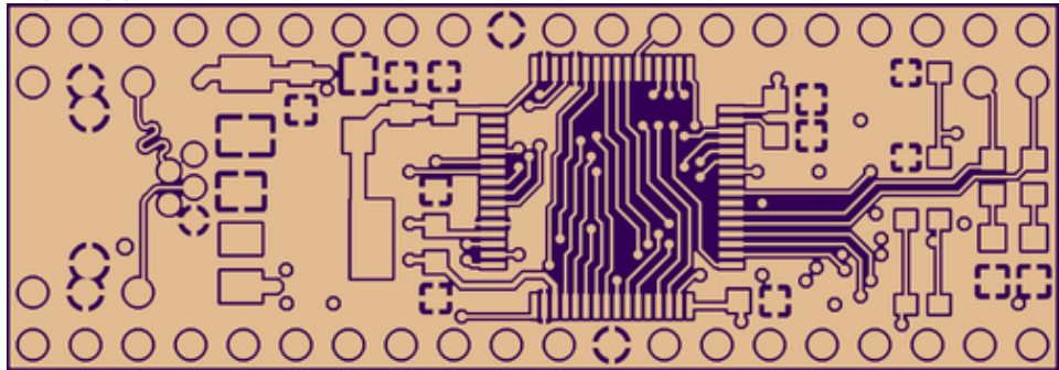
Top copper
