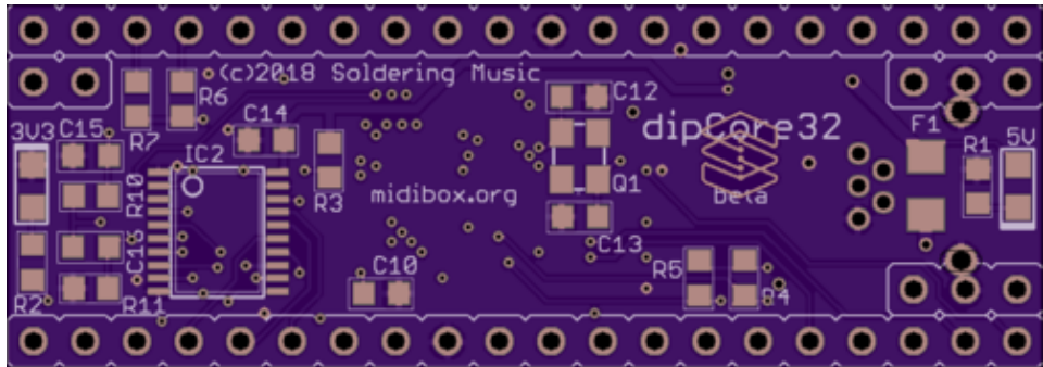
Top copper
