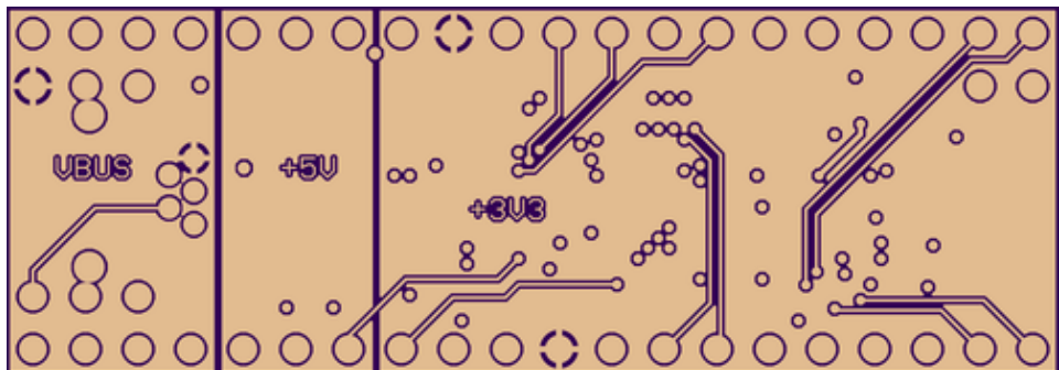
Internal 1
