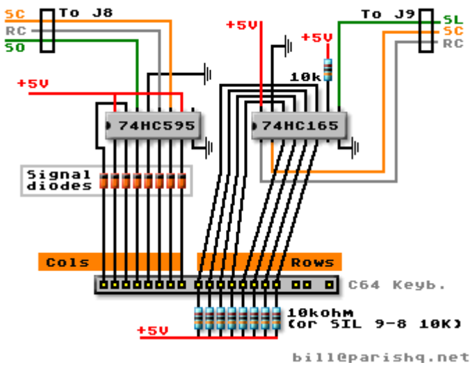
C64 Keyboard connection to MBHP v2
