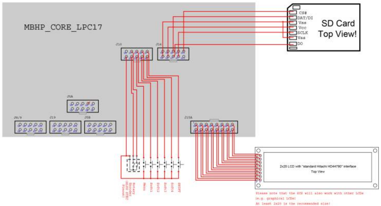
Wiring Diagram for MIDIbox NG SCS (C) T. Kloese 2013-01-02
